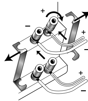
Figure 9. Loosen the terminals and remove the strapping bars that connect the two sets of terminals.
